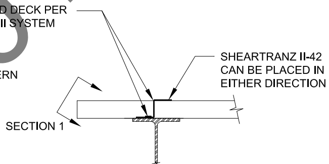
DETAIL AT DIAPHRAGM PERIMETER
